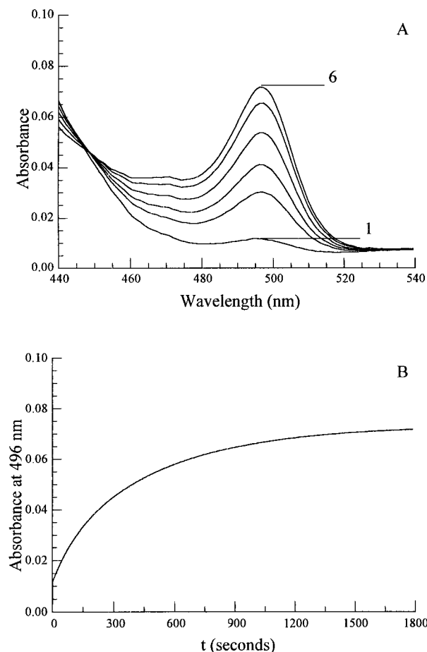
Figure 3. (A) Rapid-scanning stopped-flow spectra of the reaction of 1 mM (2 S ,3 S )- erythro - \beta -methyl-L-kynurenine and 10 mM benzaldehyde with 7 mM kynureninase in 50 mM potassium phosphate, pH 7.8. Scans were collected at 1 s intervals. The scans shown were collected at (1) 3 s, (2) 120 s, (3) 240 s, (4) 480 s, (5) 960 s, and (6) 1800 s. (B) Time course of the reaction at 496 nm.
