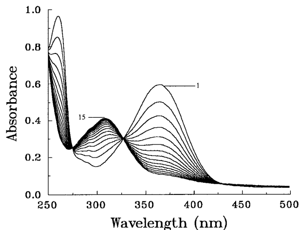
Figure 2. Reaction of (2 S ,3 S )- erythro - \beta -methyl-L-kynurenine with kynureninase. The reaction mixture contained 0.15 mM (2 S ,3 S )- erythro - \beta -methyl-L-kynurenine in 50 mM potassium phosphate, pH 7.8, and 2.8 mM kynureninase at 25°C. Scans were taken every 15 min.
