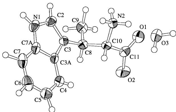
Figure 1. Structure of (2 S ,3 R )- threo - \beta -methyl-L-kynurenine hydrate.
